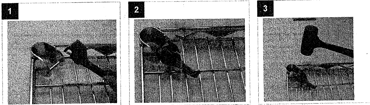
Figure B: Installing a Super Adjustable Corner Release
